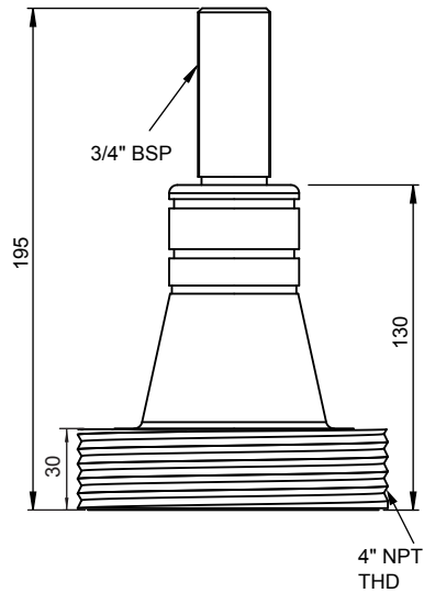
MA-WG04 with MA-WG14 window
