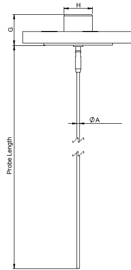
Flanged Bush
