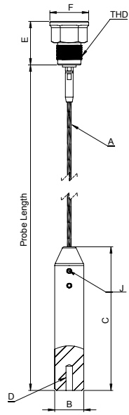
Threaded
