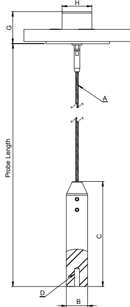
Flanged Bush
